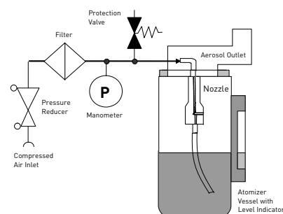
Schematic of the Atomizer Vessel with Level Indicator
